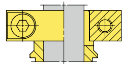
Clamping ring
