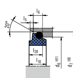
G606 EN 12756 (for eRMG1.. only)
