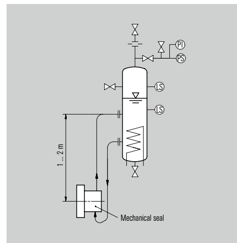
Operating and installation diagram for a TS6000 system.
