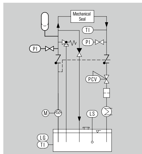
Operating and installation diagram for a SPA system with a DHE .
