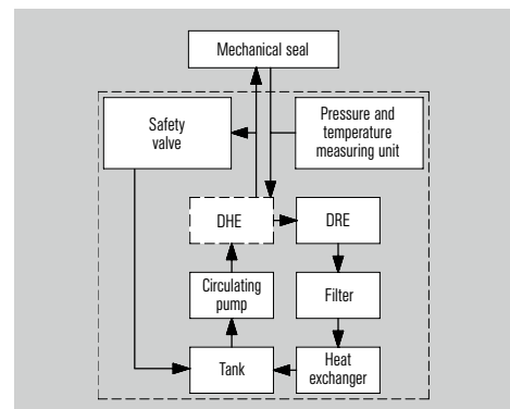
Installation and operating diagram for a SPA system
