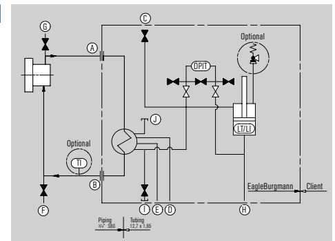
Operating and installation diagram for SPO (Plan 53C)
