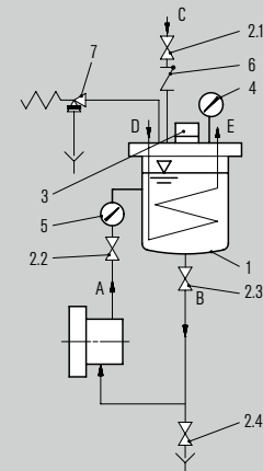
Operating and installation diagram for a TS3000 system
