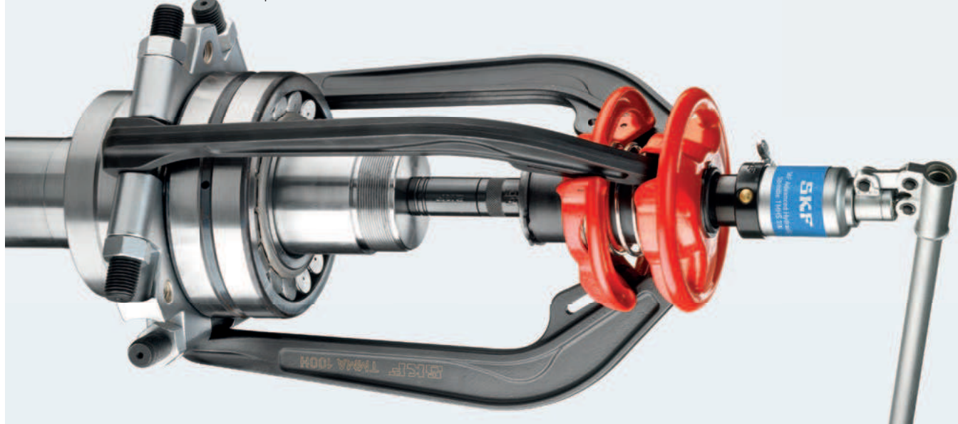
TMMS 160 shown as part of hydraulic puller set TMAA 100H/SET
